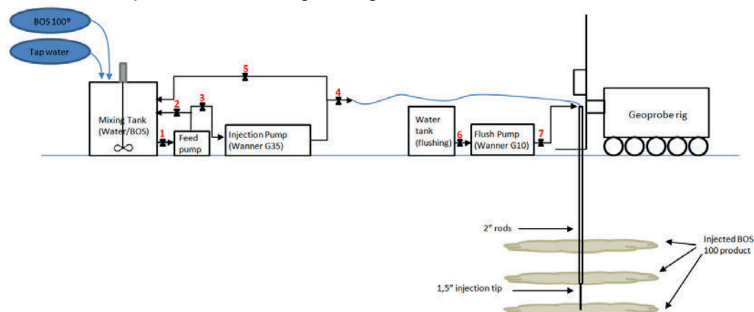
Figure 1 Schematic diagram of the injection system, drill rig, and subsurface.
